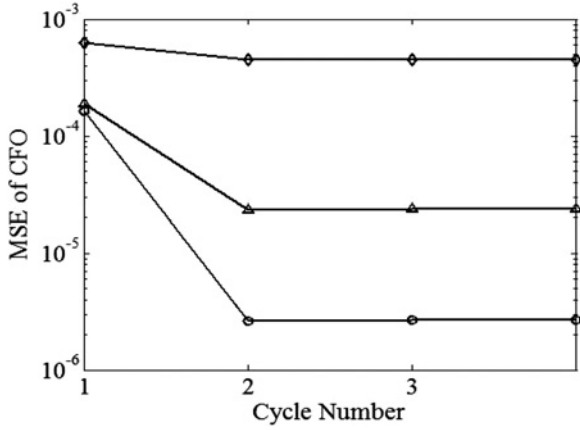
Fig. 3 MSE of CFO, -\circ- : SNR_I = 30 dB, -\Delta- : SNR_I = 15 dB, -\diamond- : SNR_I = 0 dB
