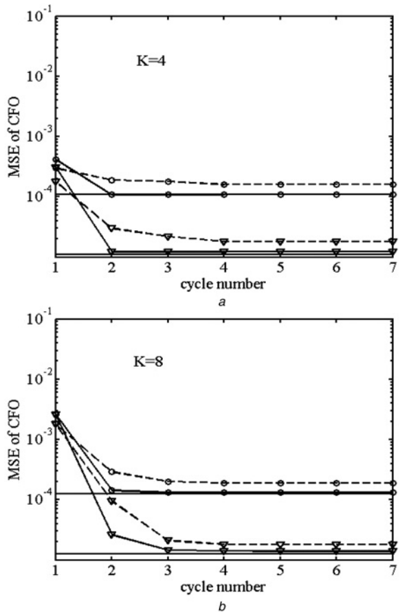
Fig. 7 Comparison on MSE of CFO, -\circ- : MSAGE at SNR = 10 dB, -\square- : efficient AP at SNR = 10 dB, -\triangle- : MSAGE at SNR = 20 dB, -\diamond- : efficient AP at SNR = 20 dB, - : CRLB
