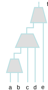
The mapped netlist
