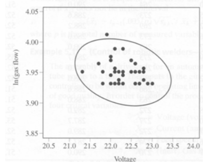
Example 5.11: 99% Quality Control Ellipse for ln(Gas flow) and voltage
