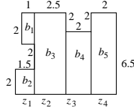
Figure 1: A concave rectilinear module consisting of four zones z_1, z_2, z_3, z_4 , where z_1 = \{b_1, b_2\} , z_2 = \{b_3\} , z_3 = \{b_4\} , and z_4 = \{b_5\} .
