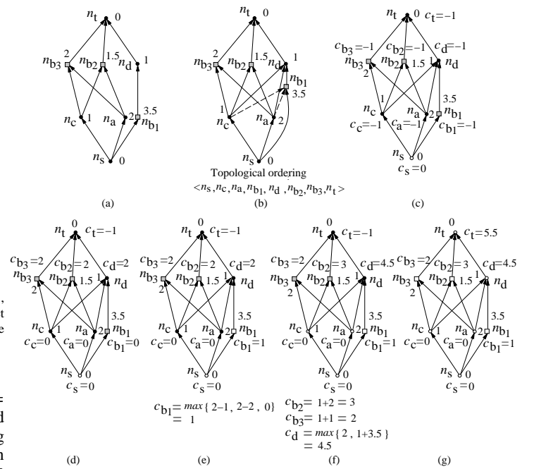
Figure 6: An example computation of Y coordinates. (a) The augmented C_v for the C_v shown in Figure 5(a). (b) The new augmented C_v after adding the edges (n_c, n_{b_1}) and (n_a, n_{b_1}) to make F_{in}(n_{b_1}) = F_{in}(n_{b_2}) = F_{in}(n_{b_3}) . A possible topological order in the new augmented C_v is given as \langle n_s, n_c, n_a, n_{b_1}, n_d, n_{b_2}, n_{b_3}, n_t \rangle . (c) The c -values of the initial configuration. (d) The c -values after relaxing the nodes n_s, n_c, n_a . (e) Before relaxing n_{b_1} , we need to compute c_{b_1}, c_{b_2} , and c_{b_3} . c_{b_1} = \max\{c_{b_2} + r(b_2, b_1), c_{b_3} + r(b_3, b_1), c_{b_1}\} = 1 . (f) c_{b_2} = c_{b_1} + r(b_1, b_2) = 3 and c_{b_3} = c_{b_1} + r(b_1, b_3) = 2 . (g) The final configuration after relaxing n_{b_1}, n_d, n_{b_2}, n_{b_3} , and n_t .
