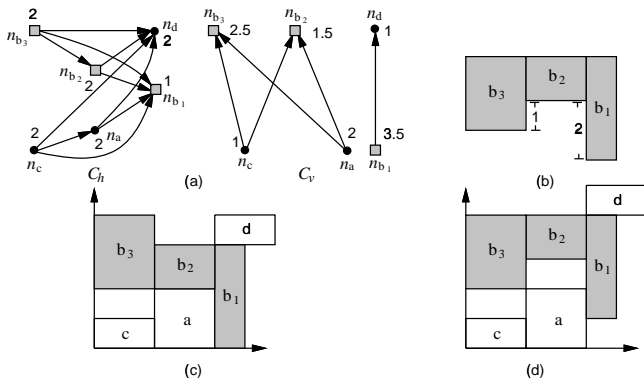
Figure 5: (a) A TCG. (b) The rectilinear module b_b consists of three submodules b_{b_1} , b_{b_2} , and b_{b_3} . (c) An incorrect packing resulting from the original packing procedure. (d) A correct packing. (Note that this packing is suboptimal; we will show in next section how to perturb the TCG to obtain an optimal packing.)
