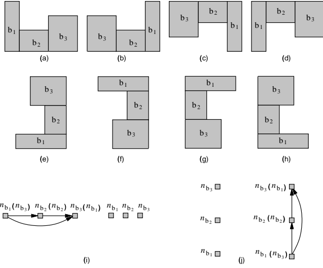
Figure 3: (a)–(h) Eight situations of the submodules for the rectilinear module b_b . (i) The subgraph of C_h and C_v for the rectilinear modules shown in (a)–(d). (j) The subgraph of C_h and C_v for the rectilinear modules shown in (e)–(h).
