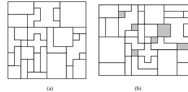
Figure 12: (a) The optimal placement (area=144). (b) The resulting placement of (a) (area=154).
