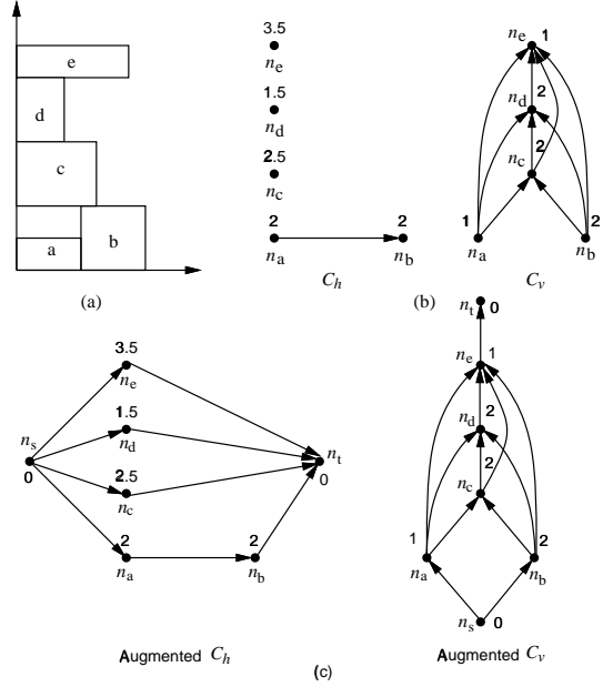
Figure 2: (a) A placement. (b) TCG. (c) Augmented TCG (augmented C_h and C_v ).
