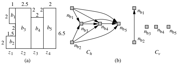
Figure 9: (a) A non-sliceable rectilinear module. (b) The components in C_h and C_v for the rectilinear module of (a).
