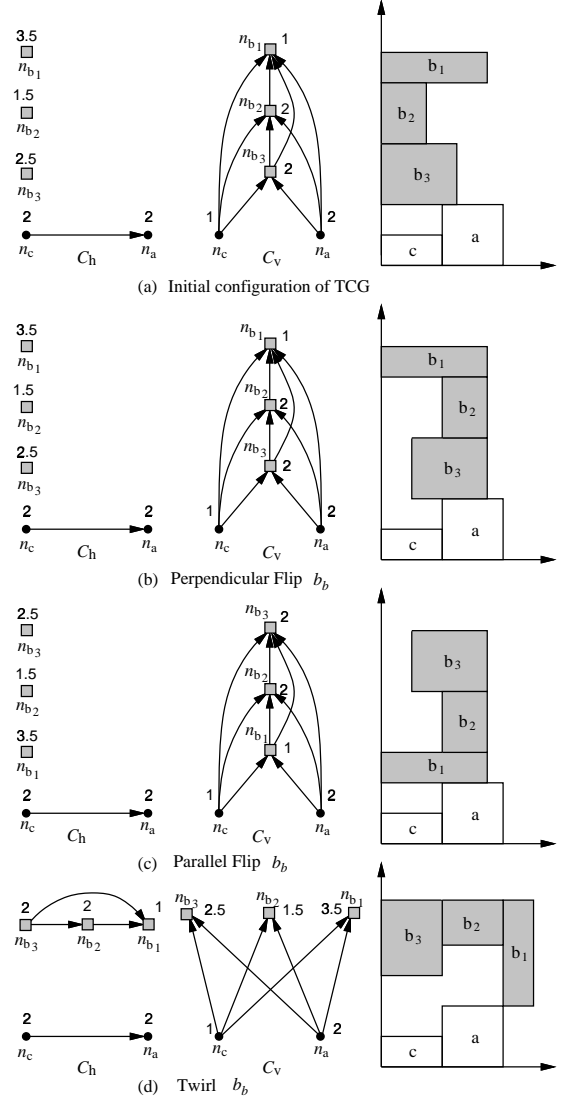
Figure 7: Examples of perturbations. (a) The initial TCG ( C_h and C_v ) and its corresponding placement. (b) The resulting TCG and placement after perpendicularly flipping the rectilinear module b_b shown in (a). (c) The resulting TCG and placement after parallel flipping the rectilinear module b_b shown in (b). (d) The resulting TCG and placement after twirling the rectilinear module b_b by -90^\circ shown in (c).
