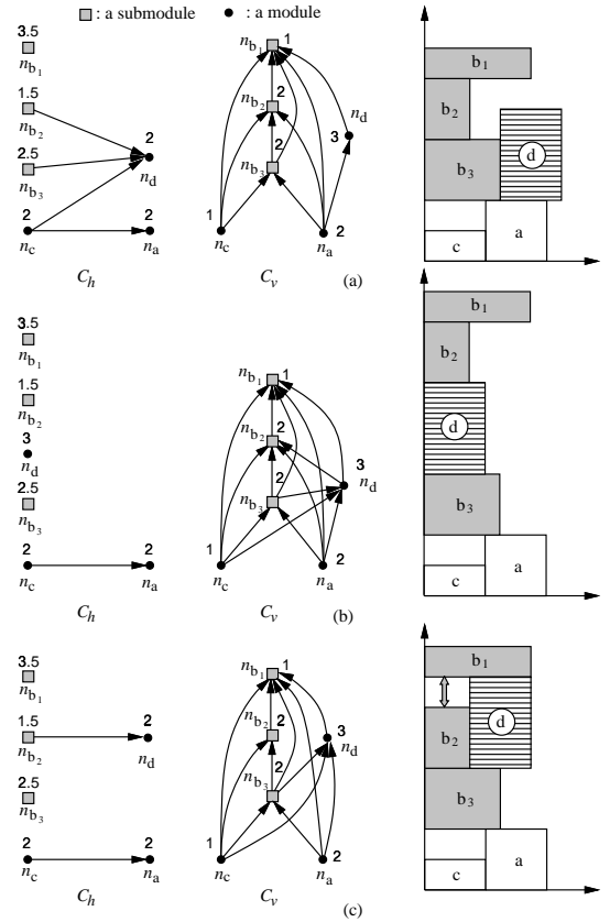
Figure 4: (a) A feasible TCG for a rectilinear module b_b and its corresponding placement. (b) A TCG that violates the inseparability constraint and its corresponding placement. (c) Expanding submodule b_{b_2} to abut with b_{b_1} . (In the figures, a quadratic node corresponds to a submodule while a round one corresponds to a rectangular module.)
