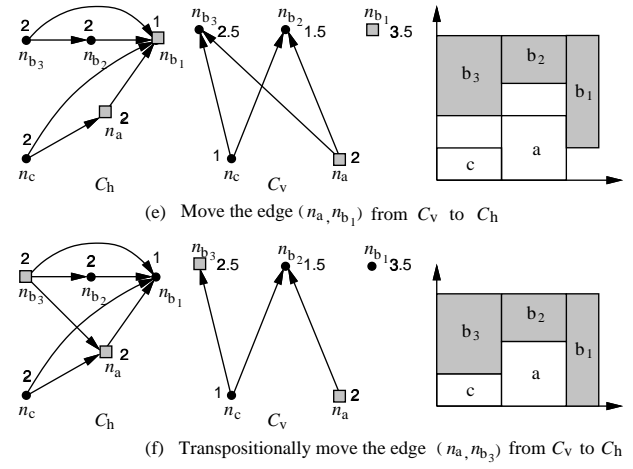
Figure 8: Examples of perturbations (continued from Figure 7). (e) The resulting TCG and placement after moving the reduction edge (na, nb_1) from the C_v of Figure 7(d) to C_h . (f) The resulting TCG and placement after transpositionally moving the reduction edge (na, nb_3) from the C_v shown in (e) to C_h .
